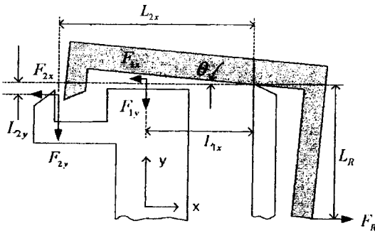
Fig. 2 Magnetic forces acting on the armature and their change with armature angle
