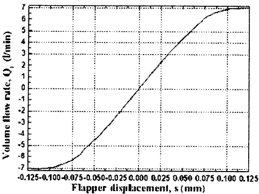
(b) No load flow rate-to-flapper displacement curve
