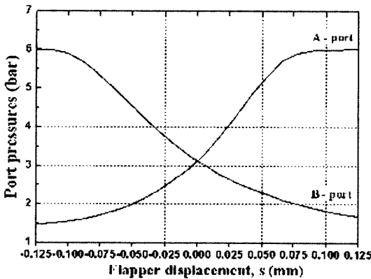
(a) Blocked load port pressures-to-flapper displacement curves
