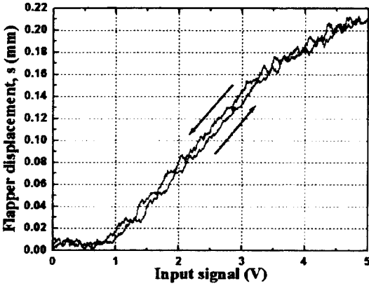
(a) Flapper displacement-to-input signal curve
