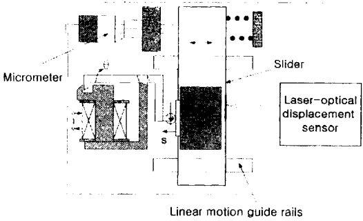
Fig. 7 Experimental setup for the force measurement
