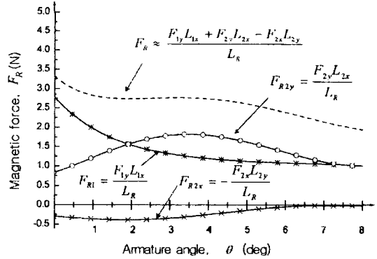
Fig. 2 Magnetic forces acting on the armature and their change with armature angle
