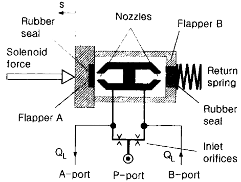
Fig. 8 Schematics of a double flapper nozzle valve for 4/3-way directional control
