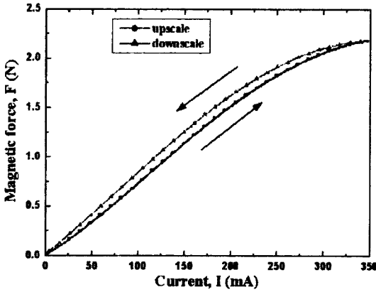
(a) Magnetic force-to-current curve
