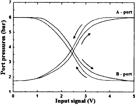
(b) Port pressures-to-input signal curves
