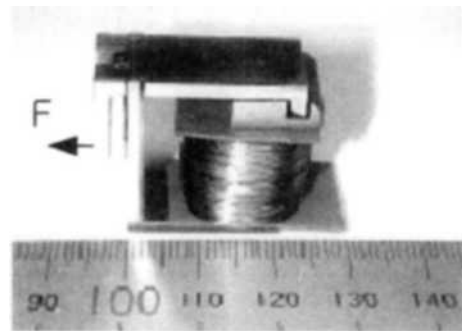
Fig. 5 Prototype of a proportional solenoid ( L_{21}=21 , L_{22}=2 , L_{11}=11.5 , L_{12}=7 , L_R=13 , H=12 (mm))
